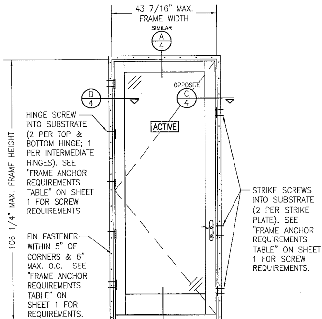
INTERIOR ELEVATION: SINGLE DOOR SCALE: 1/2" = 1'-0"
