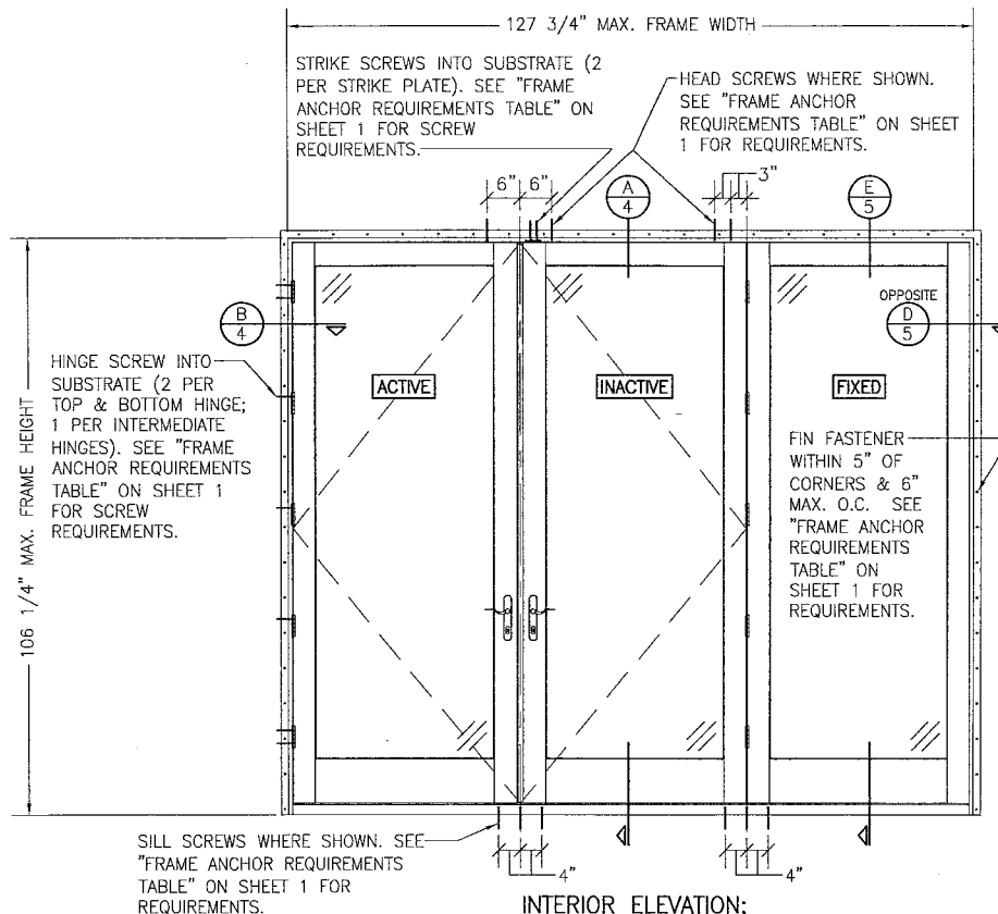
INTERIOR ELEVATION: DOUBLE DOORS WITH A FIXED PANEL DOOR SCALE: 1/2" = 1'-0"
