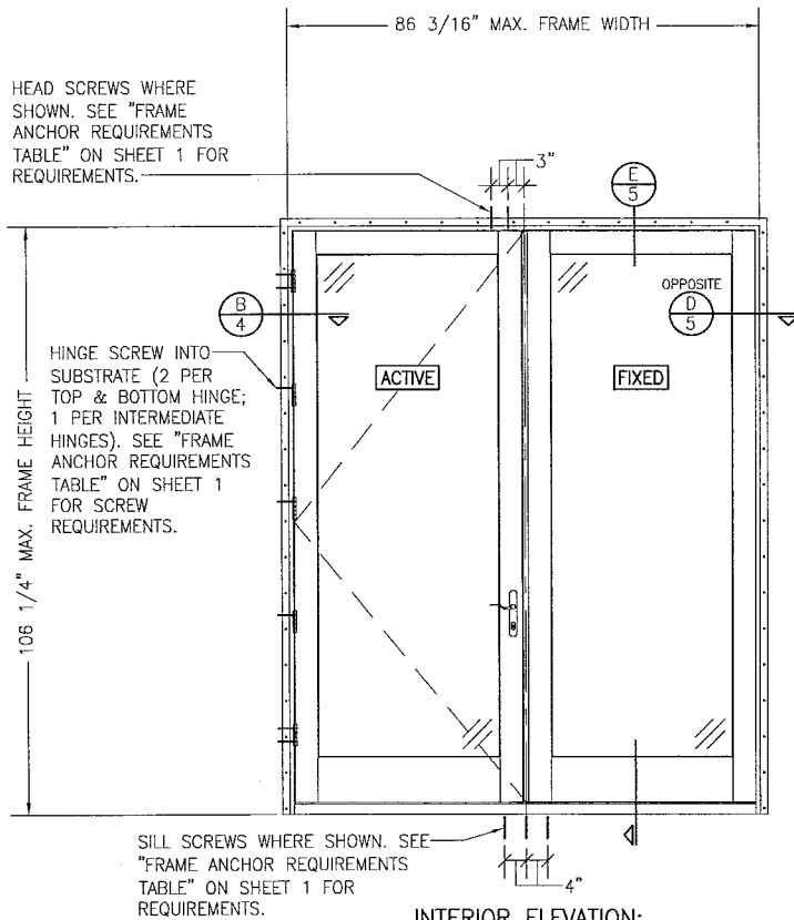
INTERIOR ELEVATION: SINGLE DOOR WITH A FIXED PANEL DOOR SCALE: 1/2" = 1'-0"
