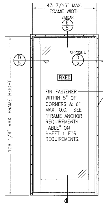
INTERIOR ELEVATION: FIXED PANEL DOOR SCALE: 1/2" = 1'-0"
